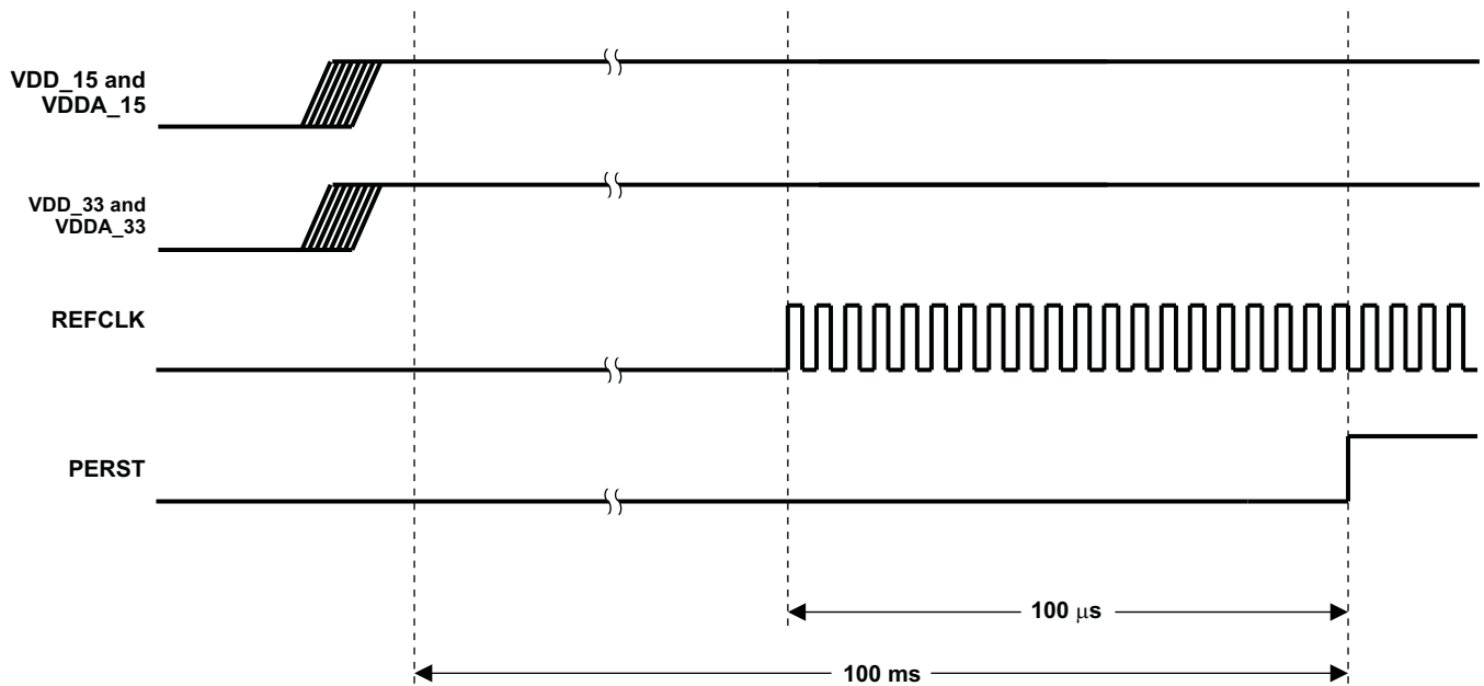
Figure 3-2. Power-Up Sequence
